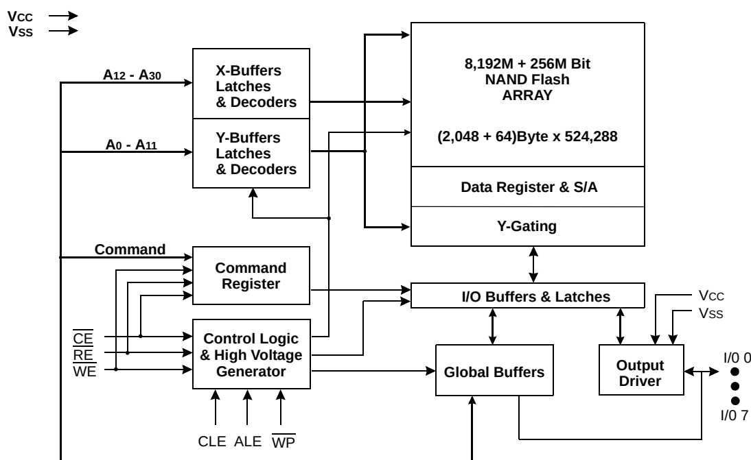
Figure 1. K9L8G08U0M Functional Block Diagram
