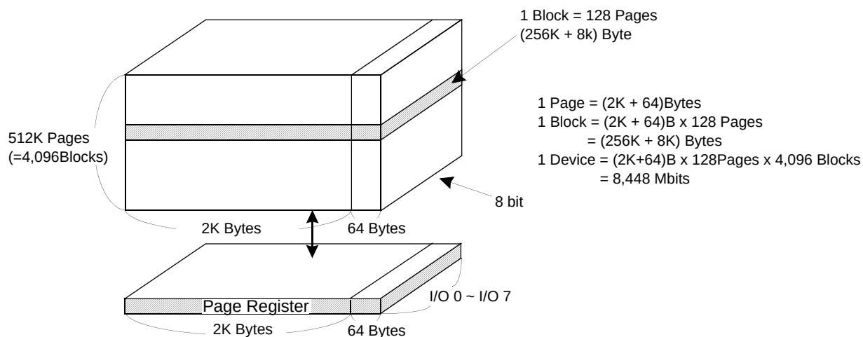
Figure 2. K9L8G08U0M Array Organization
